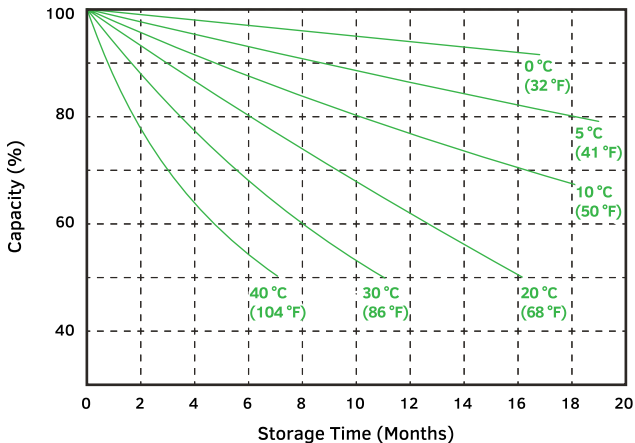
Self-Discharge characteristic
