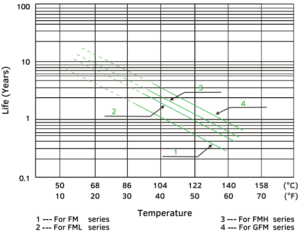
Temperature effects on float life
