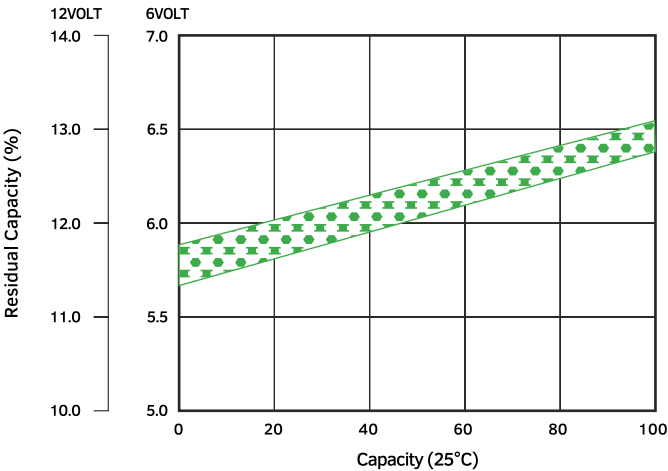
Relationship of OCV and Residual Capacity % (25°C)
