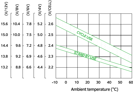
Relationship between charge voltage and temperature
