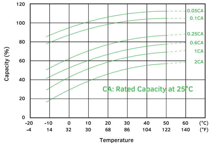
Temperature effects on capacity
