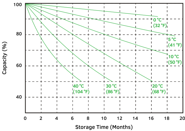
Self-Discharge characteristic
